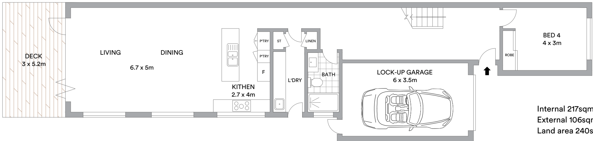
GROUND FLOOR
