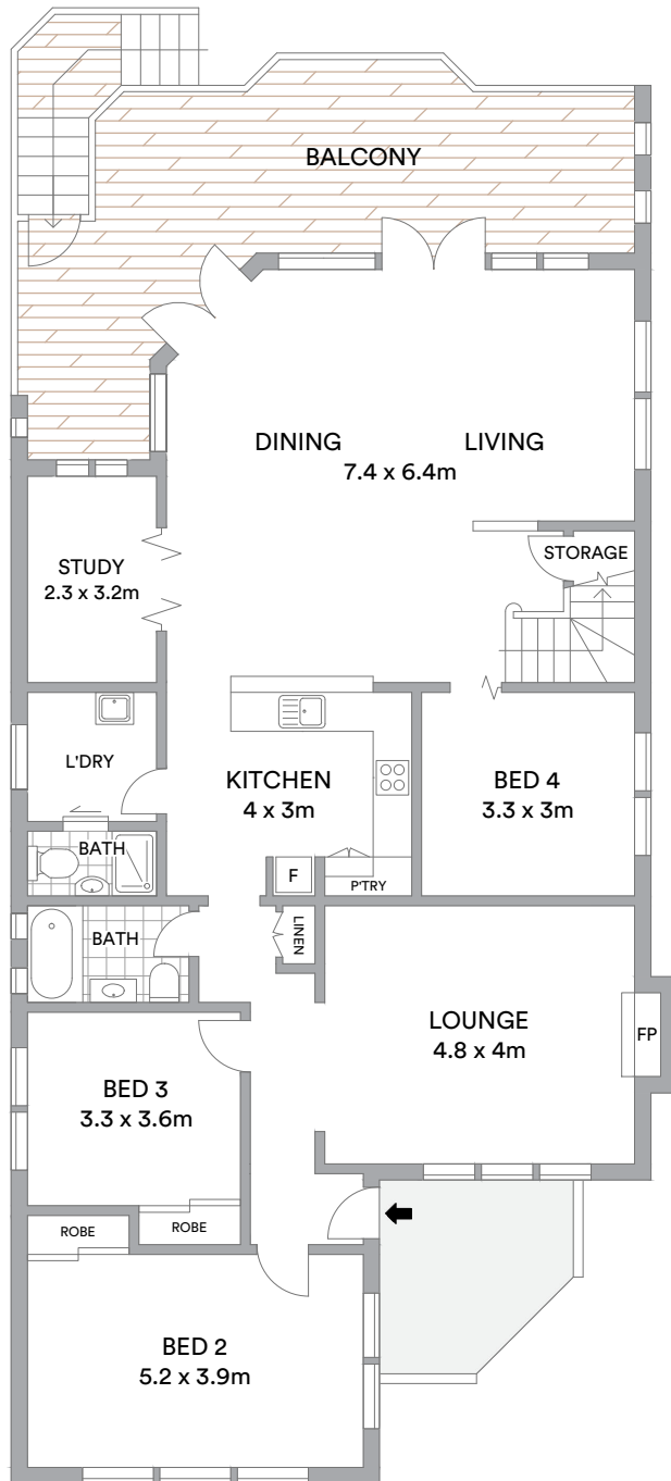
GROUND FLOOR
