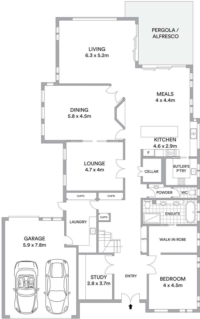
GROUND FLOOR
