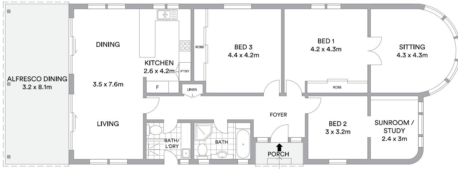
GROUND LEVEL
