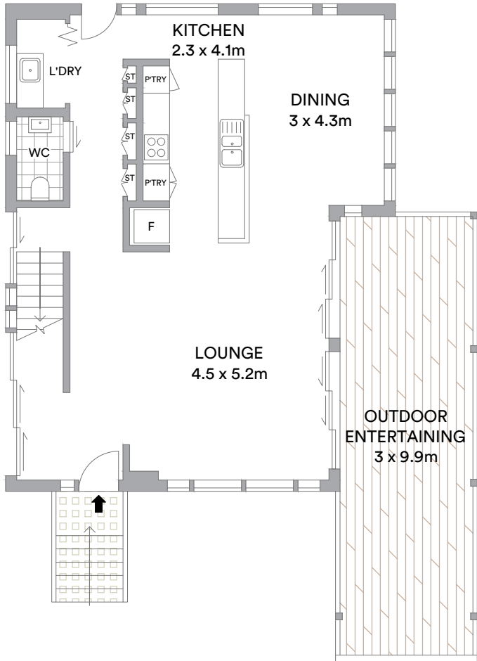
ENTRY LEVEL
